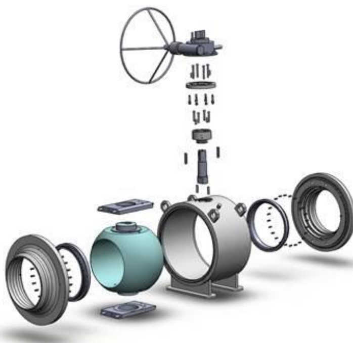
Figure 15: Exploded view of a FWBV series valve.
